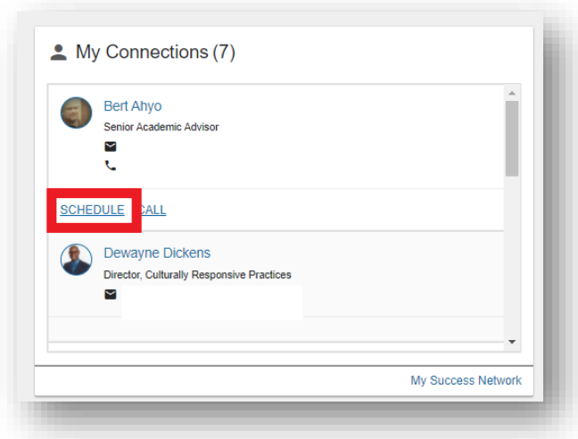
Figure 2 My Connections
